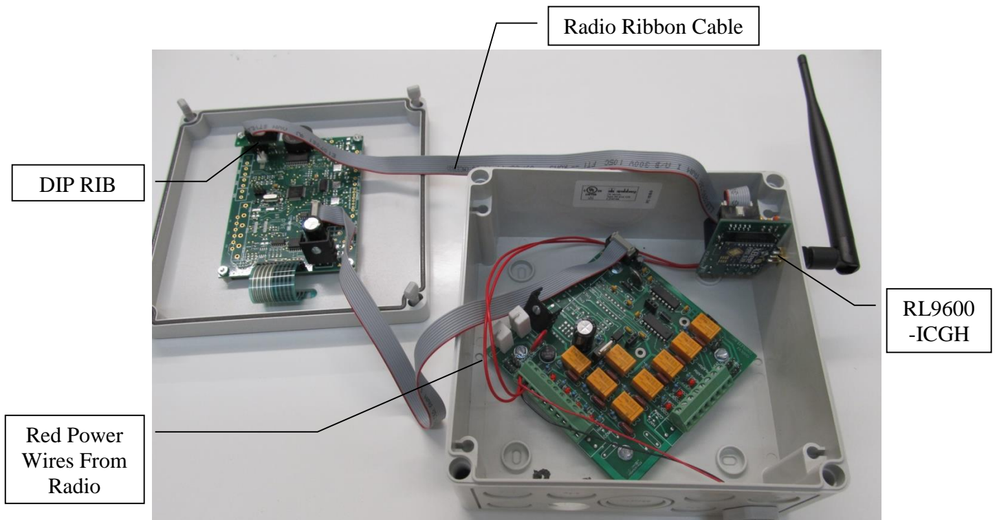
Figure 17: All power connections hooked up.
