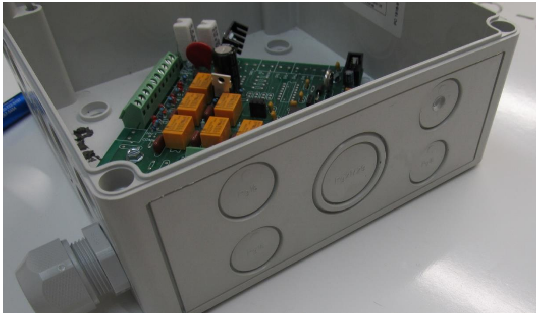
Figure 16: The hole drilled in the right, top, front knockout of the controller.
