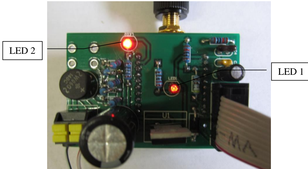
Figure 1: LED 2 will flash during the range test. LED 1 will light up when the switch is pushed to indicate power to the board.
