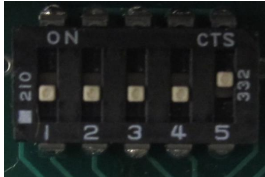
Figure 12: DIP switch 5 set to ON.
