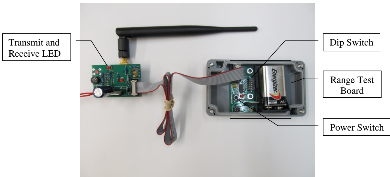
Figure 13: Wireless radio/range test configuration.
